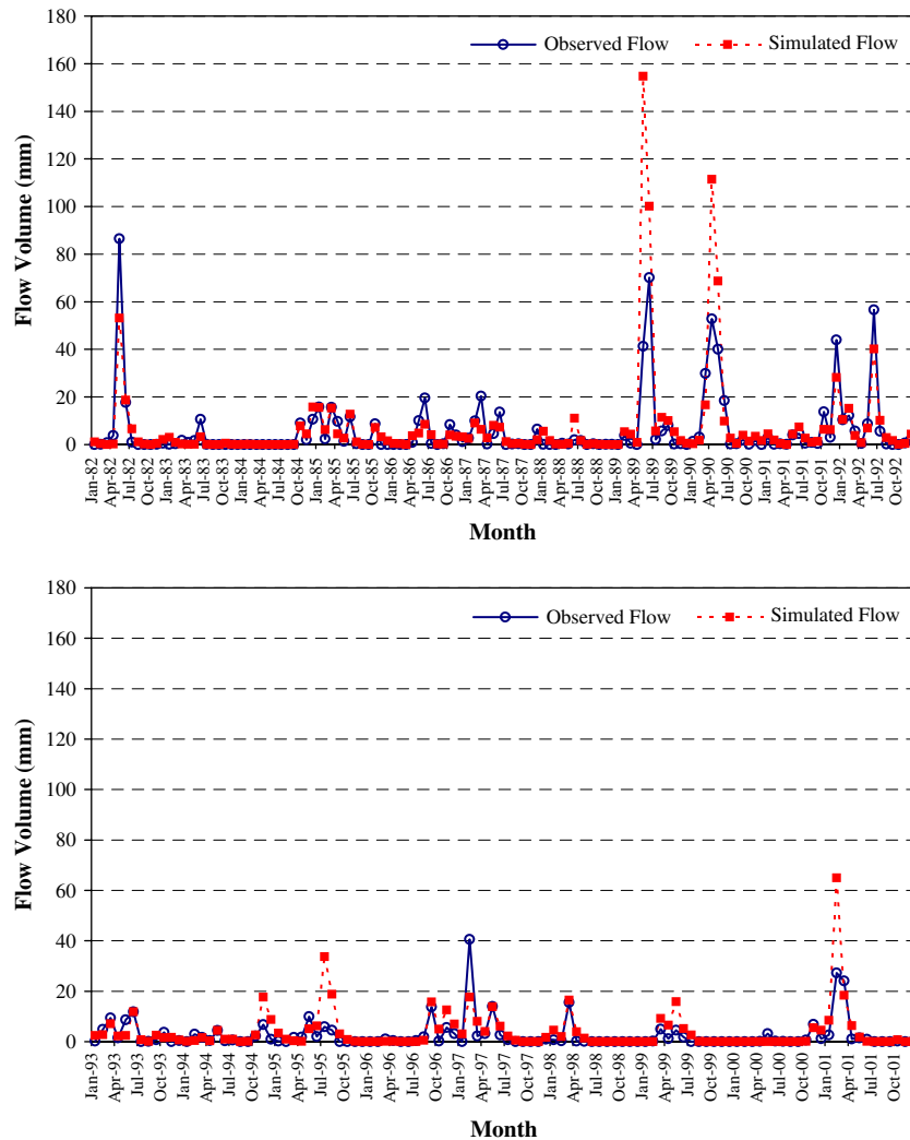
Fig. 3. Monthly observed and simulated flows near Jacksboro, Texas.
