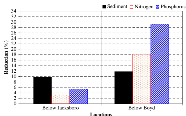
Fig. 8. Percentage reductions in sediment and nutrient loadings at two locations along the West Fork River for the additional scenario.
