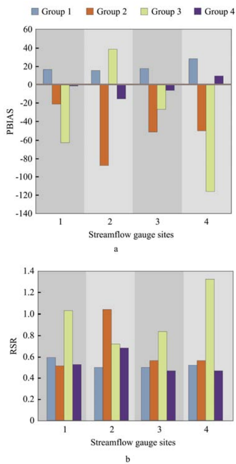
Figure 8 Bias Percentages (PBIAS) (a) and RSR (b) values between observed and simulated monthly flows
