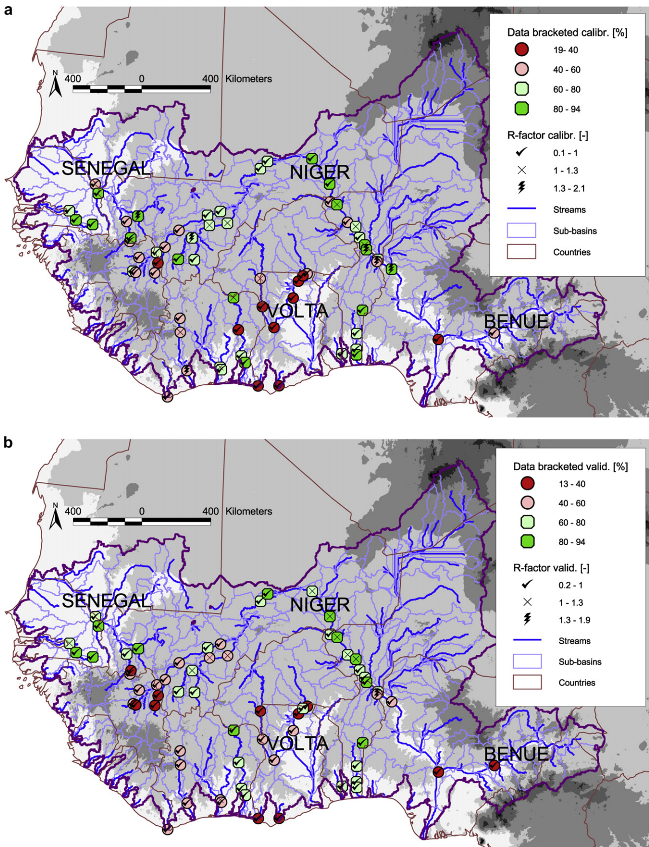
Figure 4 Measured monthly runoff data bracketed by the 95% prediction uncertainty and the R -factor of the monthly (a) calibration and (b) validation at all 64 stations.
