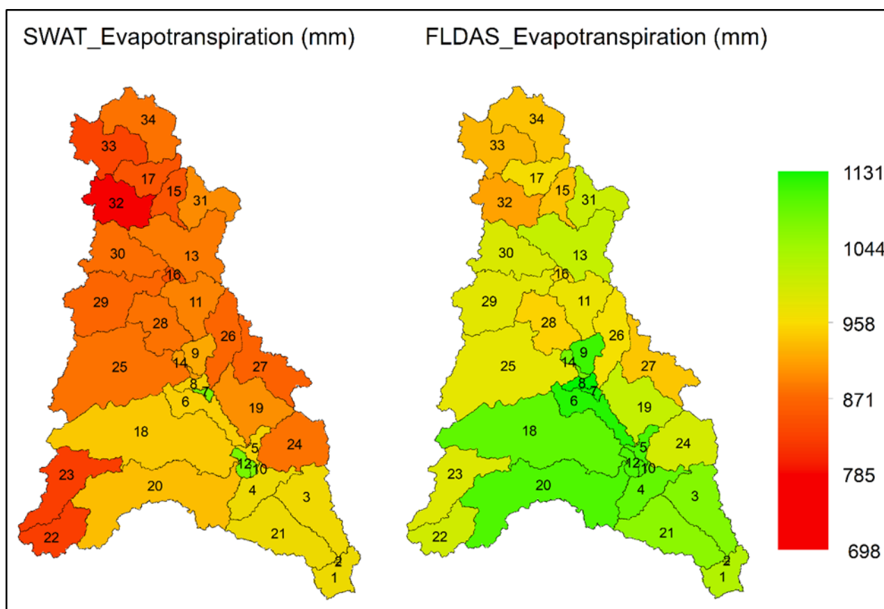
Figure 10. Spatial distribution of average annual evapotranspiration and its validation using FLDAS data over the Nagavali river basin for the period of 24 years (1991–2014).
